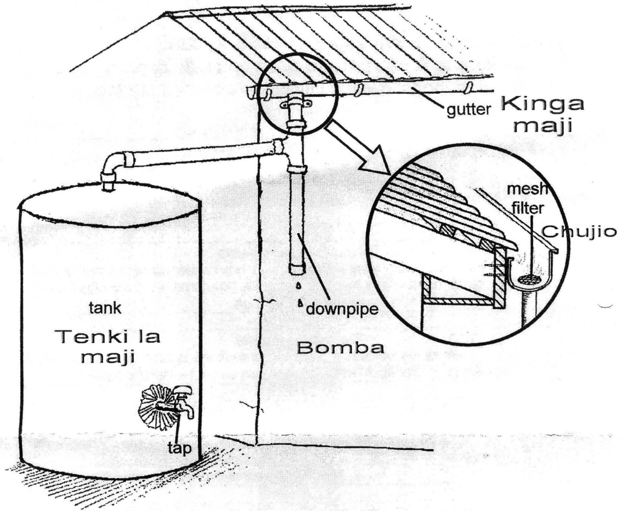
Rainwater harvesting system
